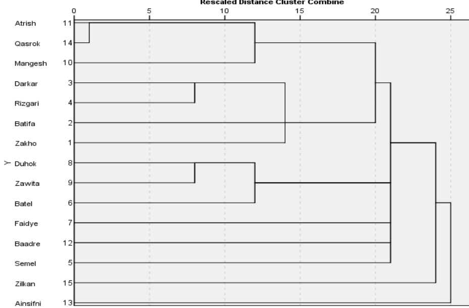
Dendrogram using Single Linkage
